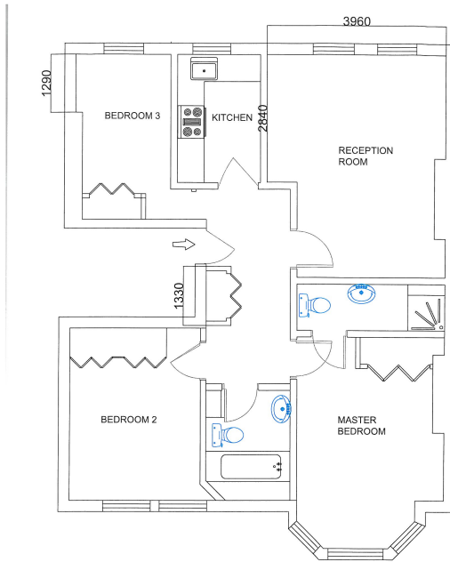
EXISTING FLOOR PLAN Scale 1:50
