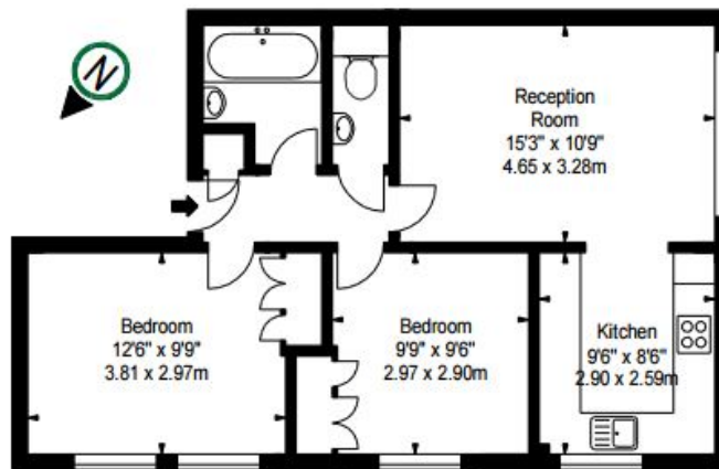
FOURTH FLOOR
